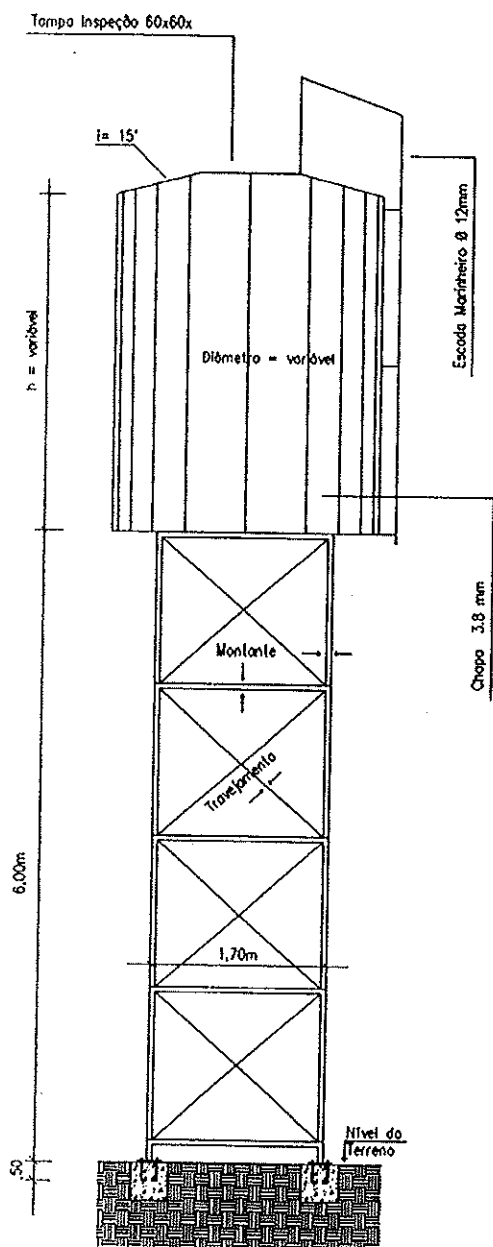
VISTA FRONTAL
